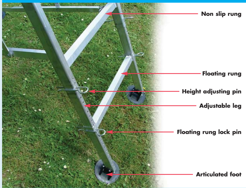
HedgeMaster on uneven ground
